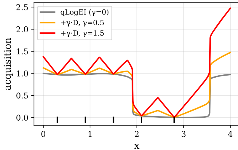
(b) DIV-qLogEI landscape
