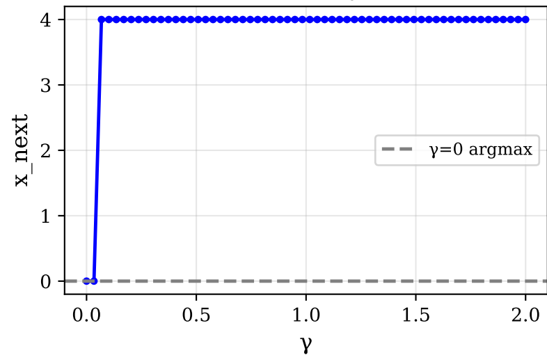
(c) Next query vs \gamma
